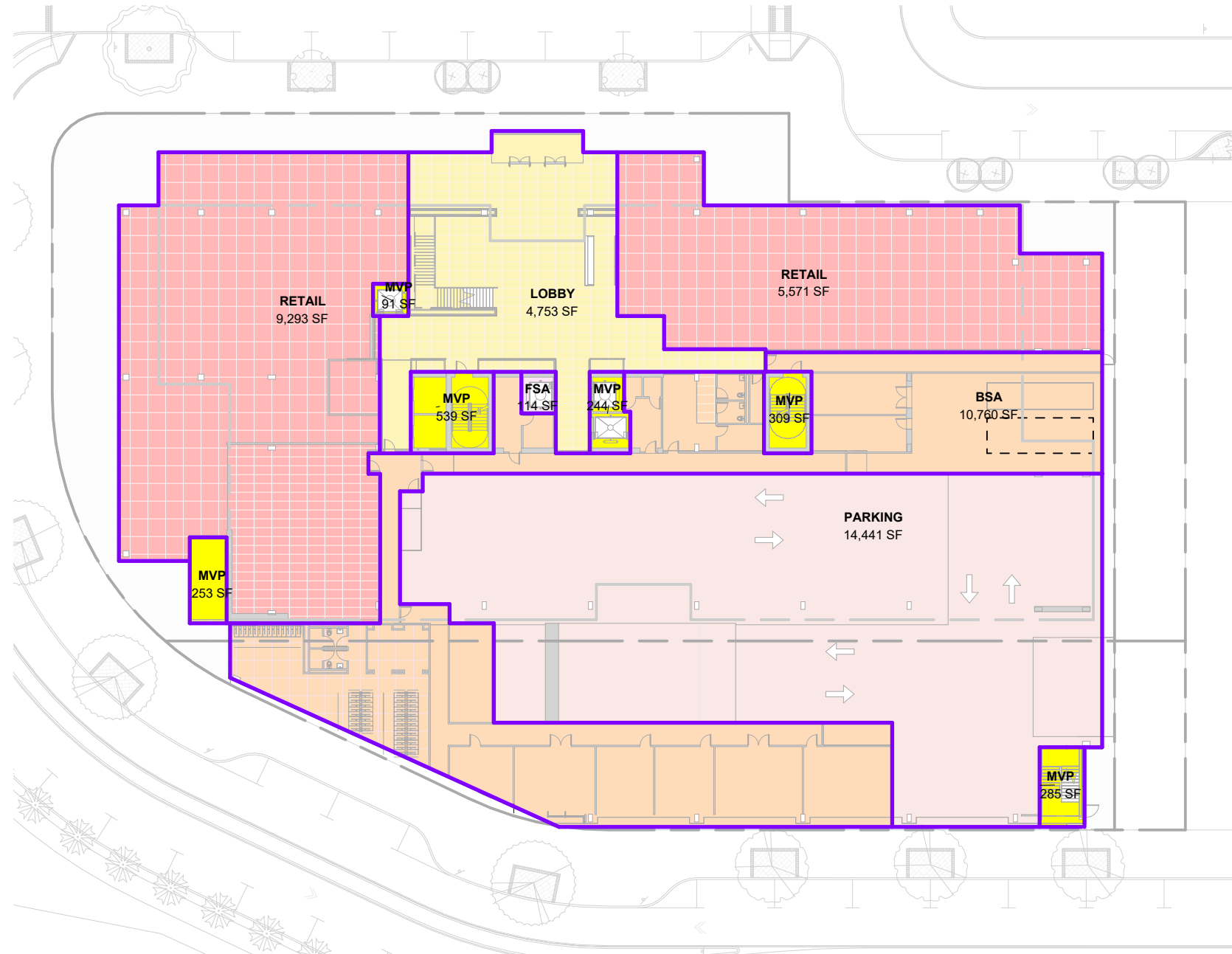
1 LEVEL 1 - LOBBY / RETAIL 1" = 40'-0"
